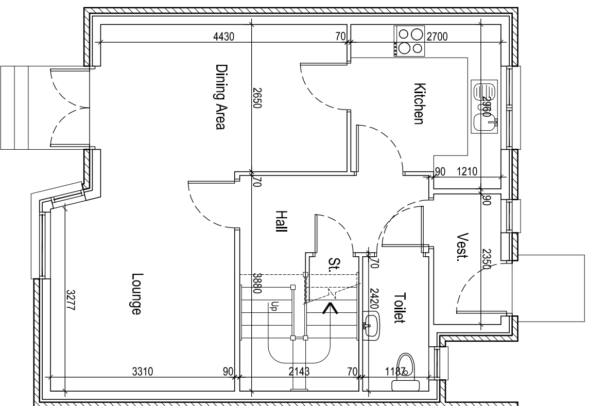
Ground Floor Plan (49.01m 2 )
